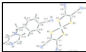
Fig. 1. Molecular structure of (I). Displacement ellipsoids are drawn at the 30% probability level ( i = -x, -y, -z ).
