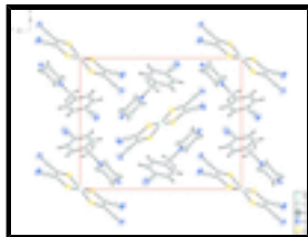
Fig. 2. Packing diagram for (I) viewed along a axis.
